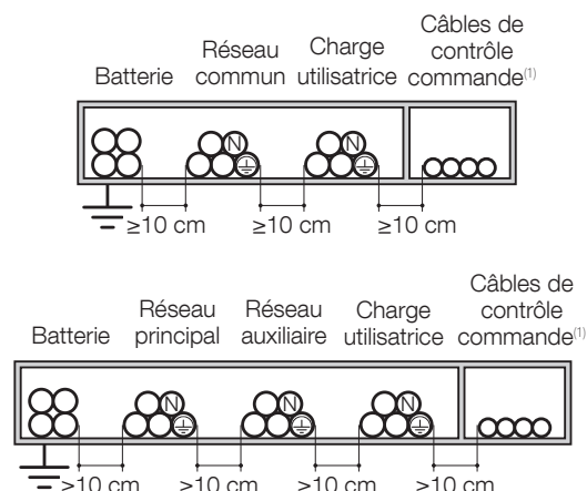
Installation acceptable
